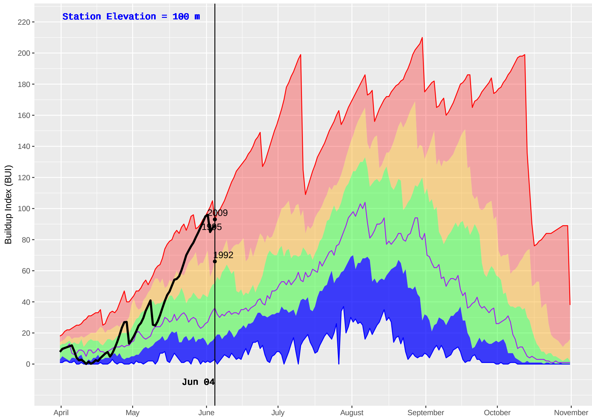
BEAVER CREEK (37) : Historical (1987–2016) and Current (2018) Noon Buildup Index (BUI)
