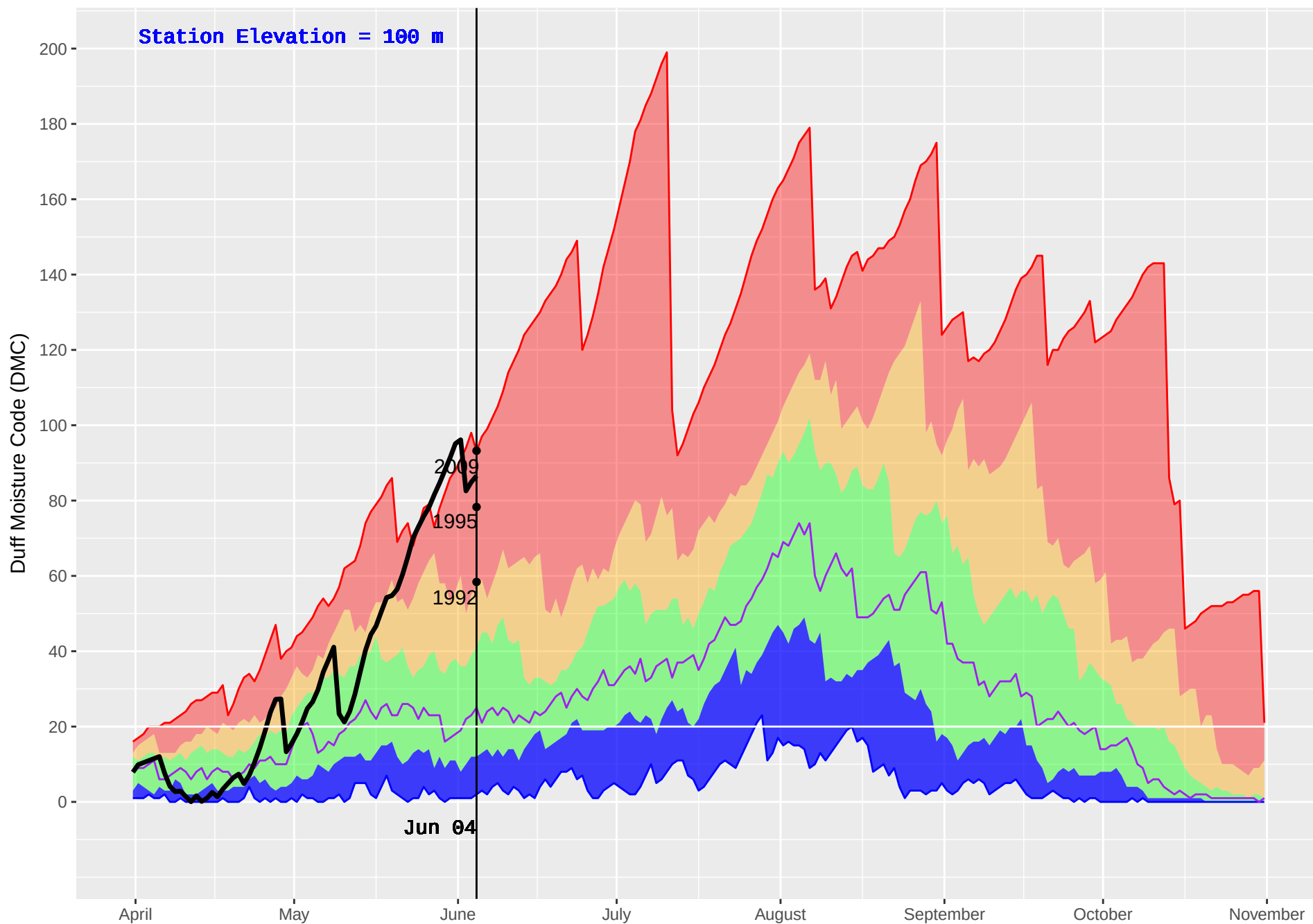
BEAVER CREEK (37) : Historical (1987–2016) and Current (2018) Noon Duff Moisture Code (DMC)
