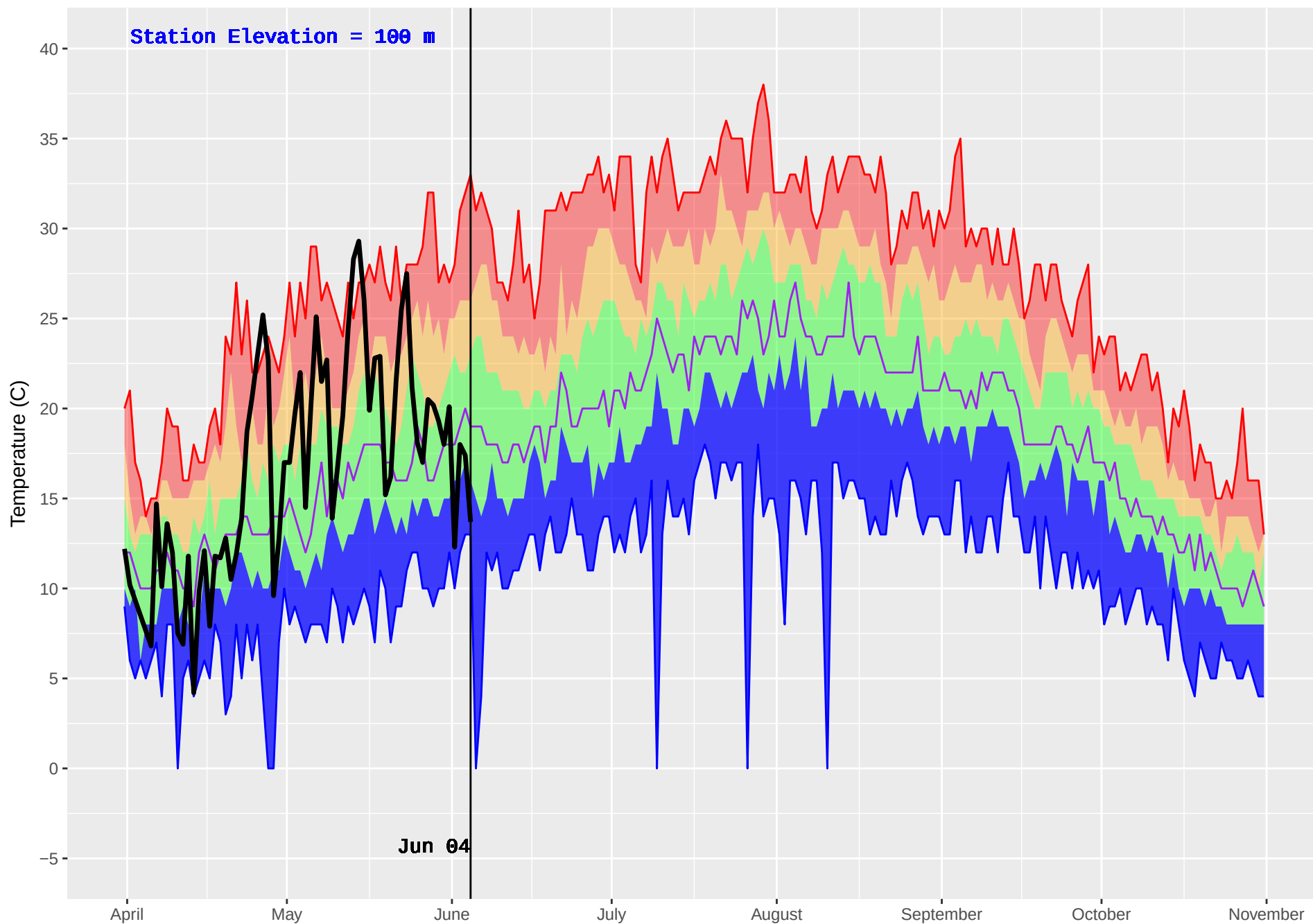
BEAVER CREEK (37) : Historical (1987–2016) and Current (2018) Noon Temperature
