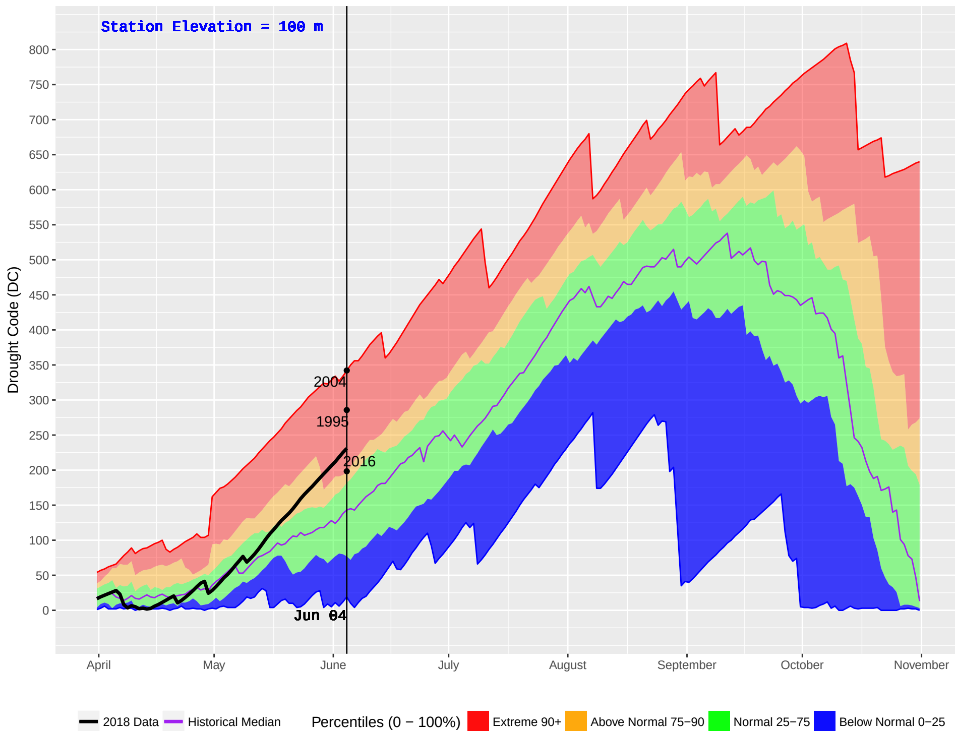
BEAVER CREEK (37) : Historical (1987–2016) and Current (2018) Noon Drought Code (DC)
